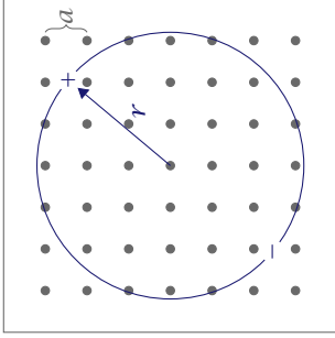
Mott-Wannier
